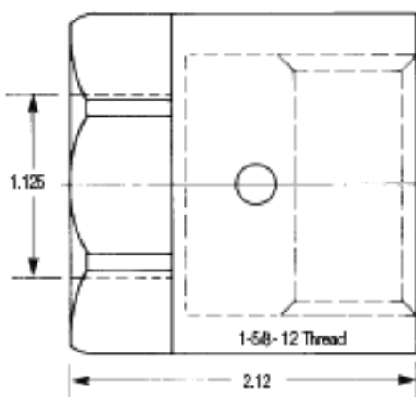
Retaining Nut Part No. H125CN- $95.
