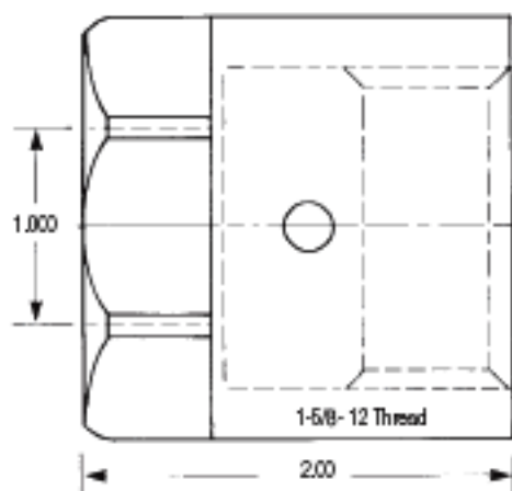
Retaining Nut Part No. H1CN- $95.
